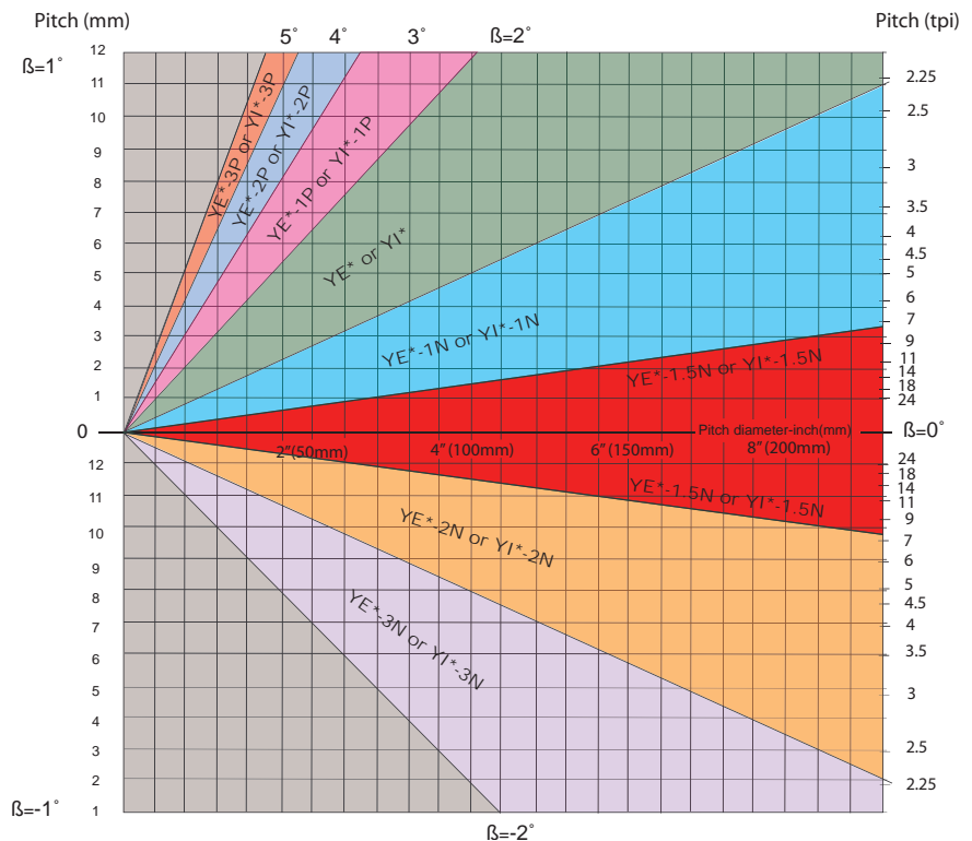
Helix Angle Diagram
